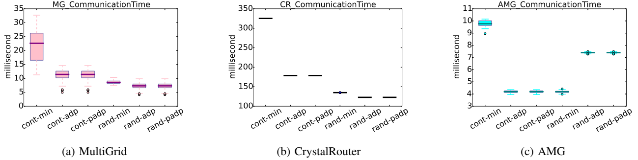
Figure 3: Communication time distribution across application ranks in Workload I.
