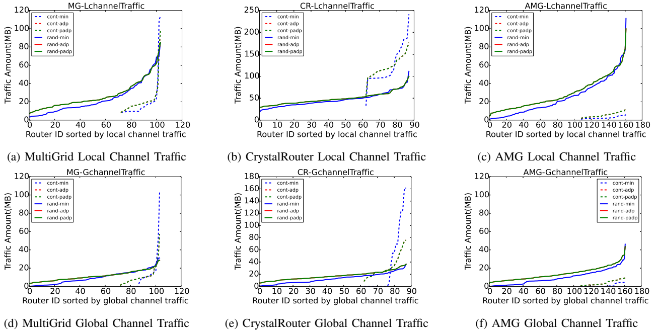
Figure 4: Aggregate workload traffic for routers serving specific applications. More routers are involved in serving each application when random placement is in use, compared to contiguous placement. In these plots, "adp" and "padp" exhibit similar behaviors, and their curves are overlapped.
