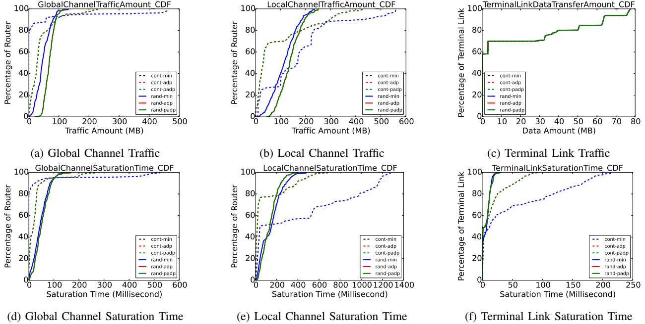
Figure 5: Aggregate traffic and saturation time for Workload II under the configurations listed in Table 1. In these plots, "adp" and "padp" exhibit similar behaviors, and their curves are overlapped.
