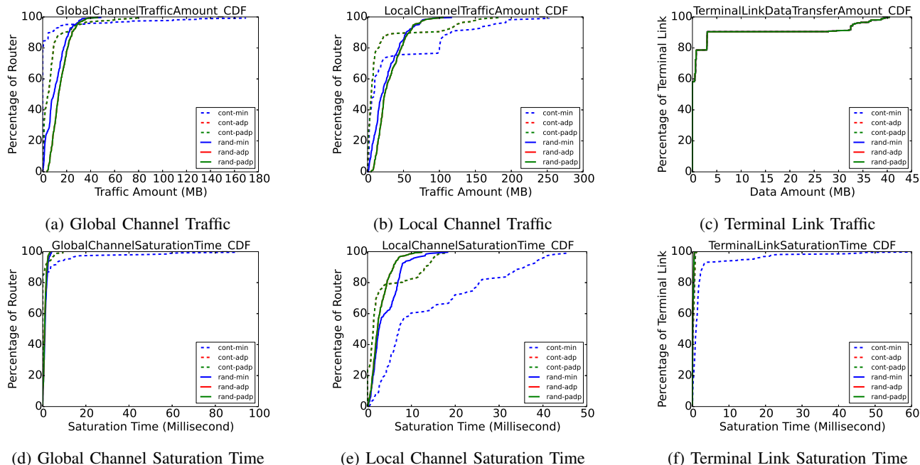
Figure 2: Aggregate traffic and saturation time for Workload I under the configurations listed in Table 1. In these plots, "adp" and "padp" exhibit similar behaviors, and their curves are overlapped.
