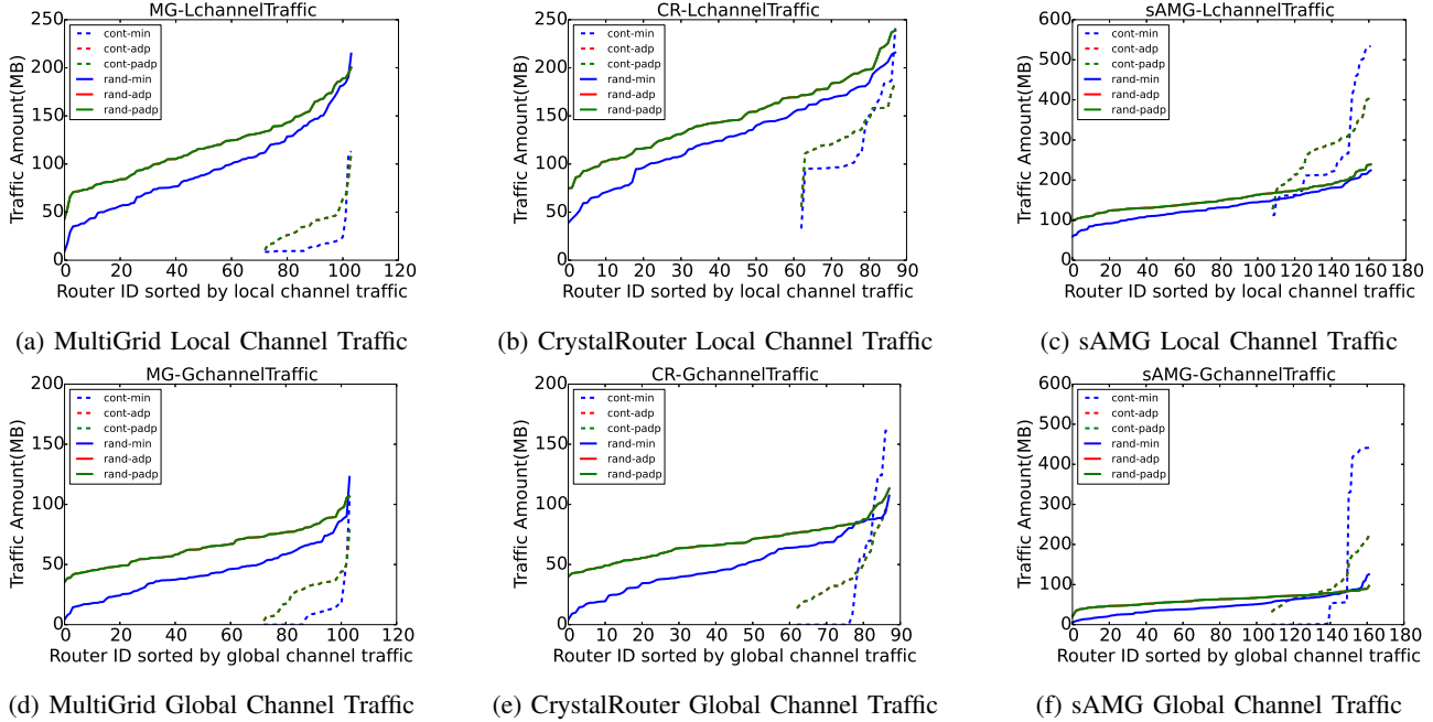
Figure 7: Aggregate workload traffic for routers serving specific applications. More routers are involved in serving each application when random placement is in use, compared to contiguous placement. In these plots, “adp” and “padp” exhibit similar behaviors, and their curves are overlapped.
