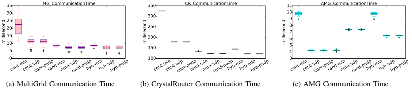
Figure 8: Application communication time. Workload I is running with all placement and routing configurations. Methods prefixed with “hyb” represent the hybrid allocation approach.
