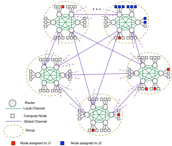
Figure 1: Five group slice of a 19-group dragonfly network. Job J_1 is allocated using random placement, while Job J_2 is allocated using contiguous placement.
